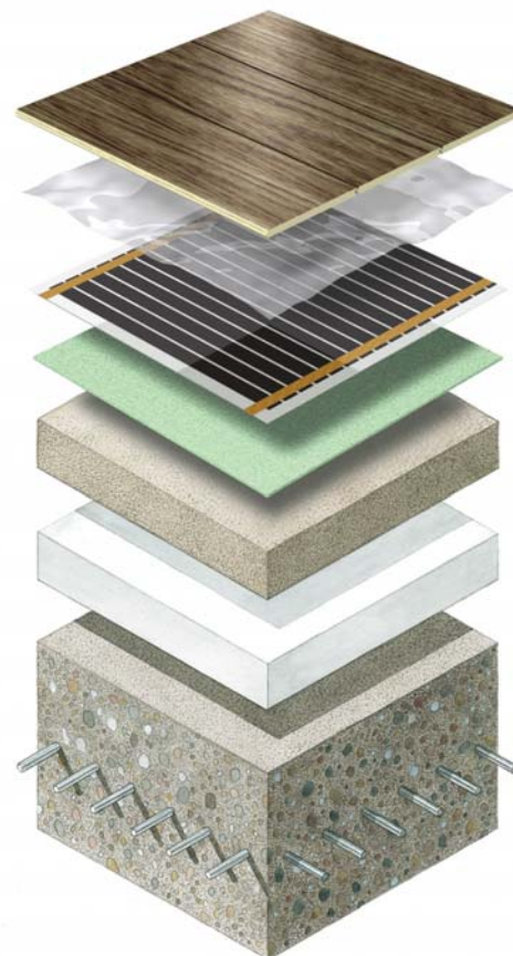
Use of Thermonet Foil in a solid floor application.
