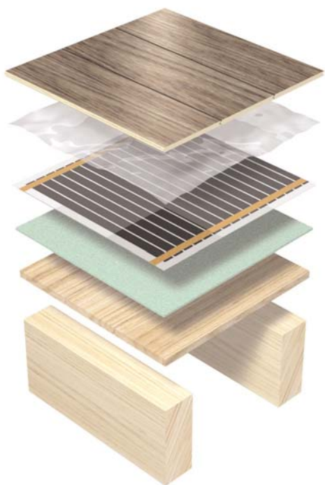
Use of Thermonet Foil in a suspended floor application.
